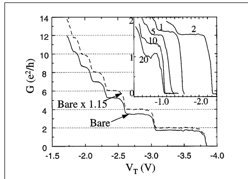
Linear response conductance of a 2 \mu\text{m} log wire in a 25 \text{ nm} quantum well vs. the top-gate voltage ( V_T ) measured at a temperature 0.3 \text{ K} . Solid line is the measured conductance. The dashed curve is the measured conductance multiplied by an empirical factor 1.15 . Inset: Linear response conductance of the last plateau for wires of different lengths fabricated consecutively along the edge of a single 25 \text{ nm} cleaved edge overgrowth specimen. The numbers denote the wire lengths in microns.
