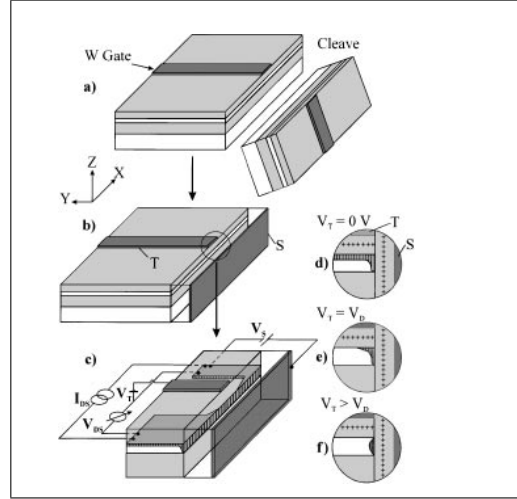
(a) Wire preparation by cleaved edge overgrowth of GaAs-AlGaAs by MBE. The wire is fabricated by cleaving the specimen [see also panel (b)]. Edge states (d) form the quantum wire. Panels (e) and (f) show different charge distributions for different top voltages. The panel (c) shows a blowup of critical device region. The mean free path is estimated as 10 \mu\text{m} , the length of the channel is about 2 \mu\text{m} .
