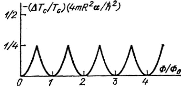
Figure 19.2: On the experiments by Little and Parks.
