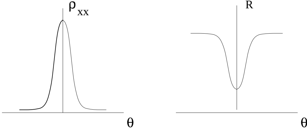
Figure 6.9: Crossover from closed to open orbits.
