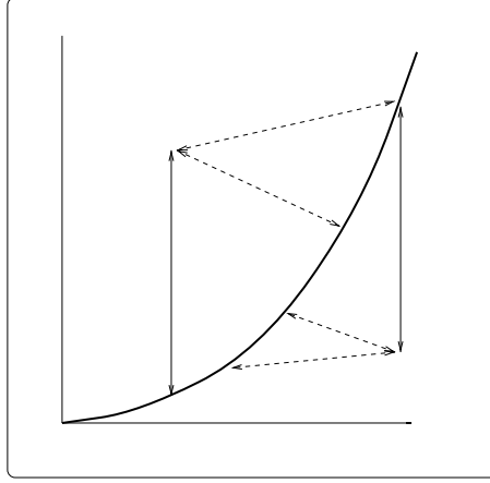
Figure 9.2: Scheme of phonon-assisted transitions. Solid curve is the electron dispersion law. Straight solid lines show optical transitions while dashed line show transistons involving phonons.
