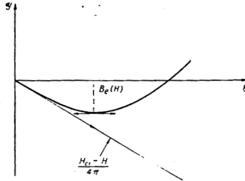
Figure 17.8: Dependence \mathcal{G} vs. B .
