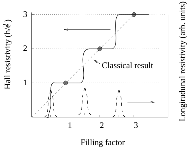
Figure 14.1: Schematic dependence of Hall resistance on filling factor.
