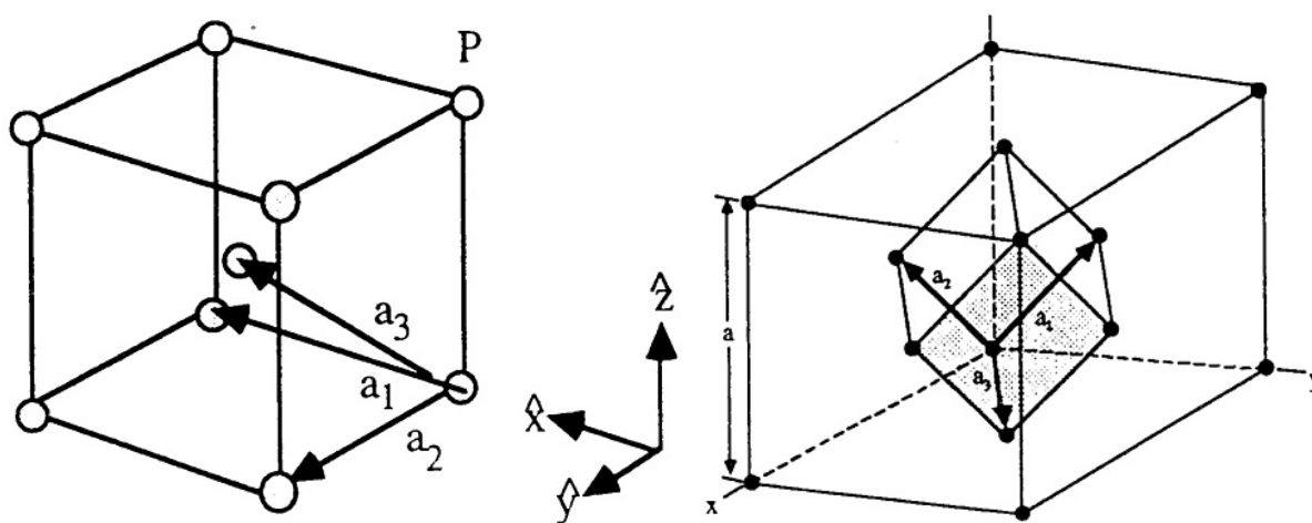
Figure 1.6: Primitive vectors for bcc (left panel) and (right panel) lattices.
