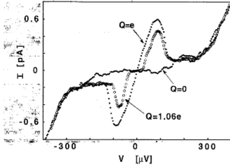
Fine scale current-voltage characteristics for Q = C_g V_g \bmod 2e = 0, e , and 1.06e . A small Coulomb gap is seen for the Q = 1.06e data.
