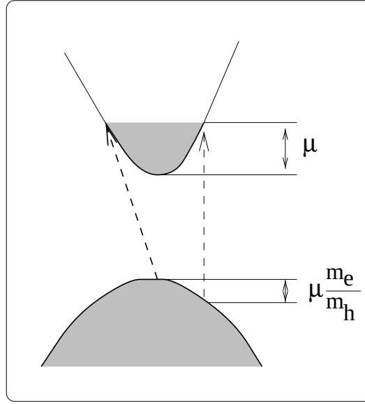
Figure 10.10: Scheme of typical interband absorption processes.
