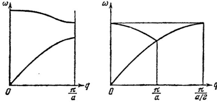
Figure 2.7: Degenerate case.
