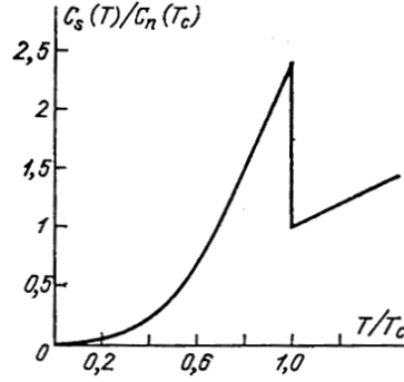
Figure 18.4: Temperature dependence of the specific heat.
