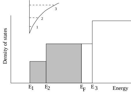
Figure 11.6: Density of states for a quasi-2D system.
