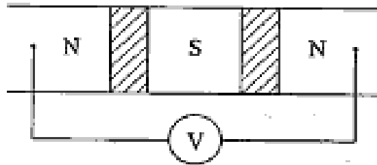
Figure 21.6: An ideal superconducting electrode between normal bulk electrodes forming two tunnel junctions in series.
