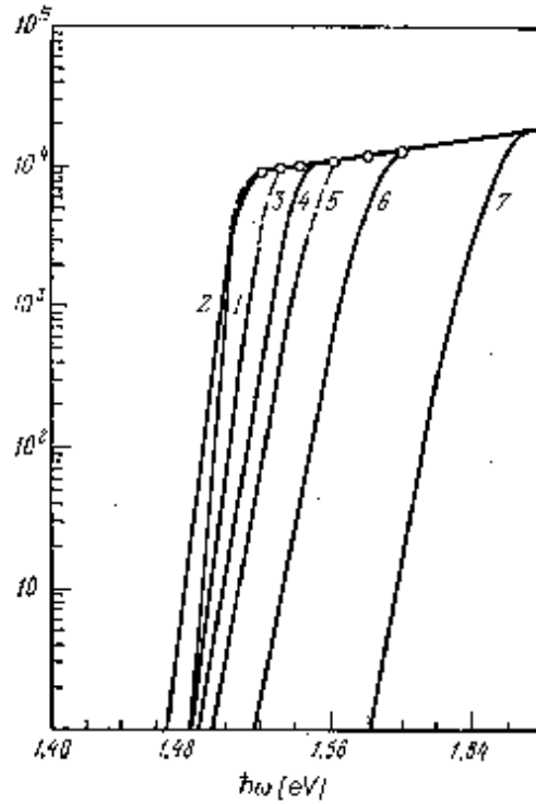
Figure 10.9: The absorption coefficient as a function of the energy of light quanta at 77 K in n -GaAs. n \cdot 10^{-17} , \text{cm}^{-3} : 1 – 0.02, 2 – 2.2, 3 – 5.3, 4 – 12, 5 – 16.2, 6 – 31.5, 7 – 65.
