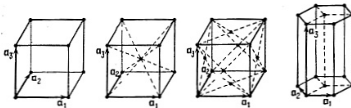
Figure 1.5: Primitive lattices
