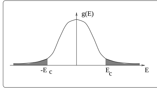
Figure 10.4: Density of states in the Anderson model. Localized states are shaded. Mobility edges are denoted as E_c .
