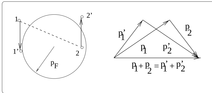
Figure 6.2: Scattering processes for electron-electron interaction.
