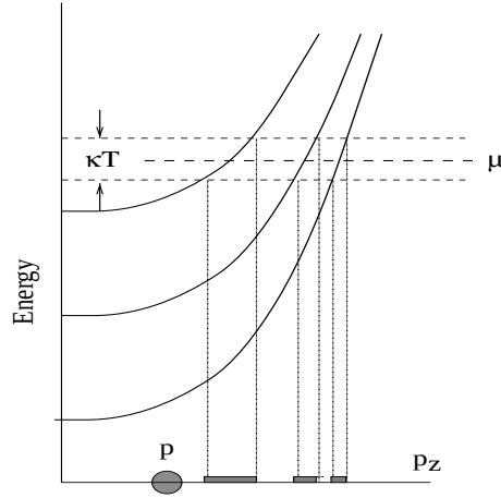
Figure 8.2: Landau levels.
