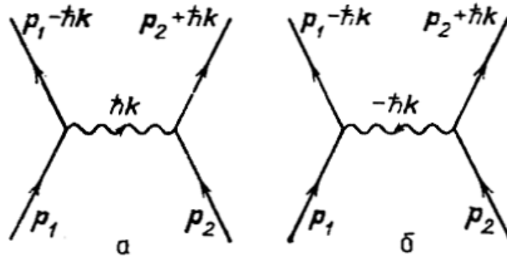
Figure 18.1: Electron-phonon processes.
