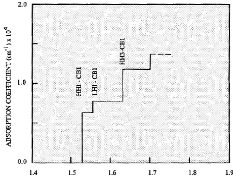
Figure 9.6: The same for 100 Å GaAs/Al 0.3 Ga 0.7 As quantum well structure for in-plane polarized light. The HH transition is \approx 3 times stronger than LH transition in this polarization. The higher sub-bands become closer spaced and eventually one gets bulk absorption coefficient.
